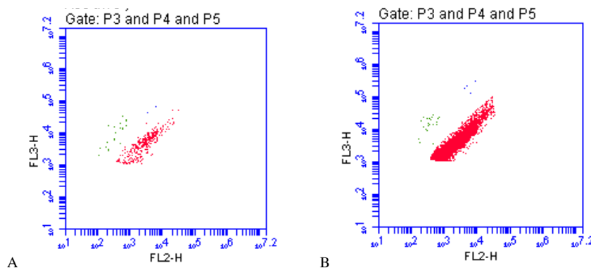
Figure 3. The flow cytometric cytogram of cell population for Şile (A) and Kızılırmak (B) Stations.
