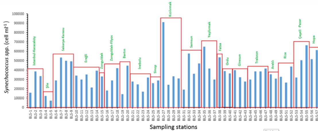
Figure 4. Synechococcus spp. cells concentration per ml in sampling station.
