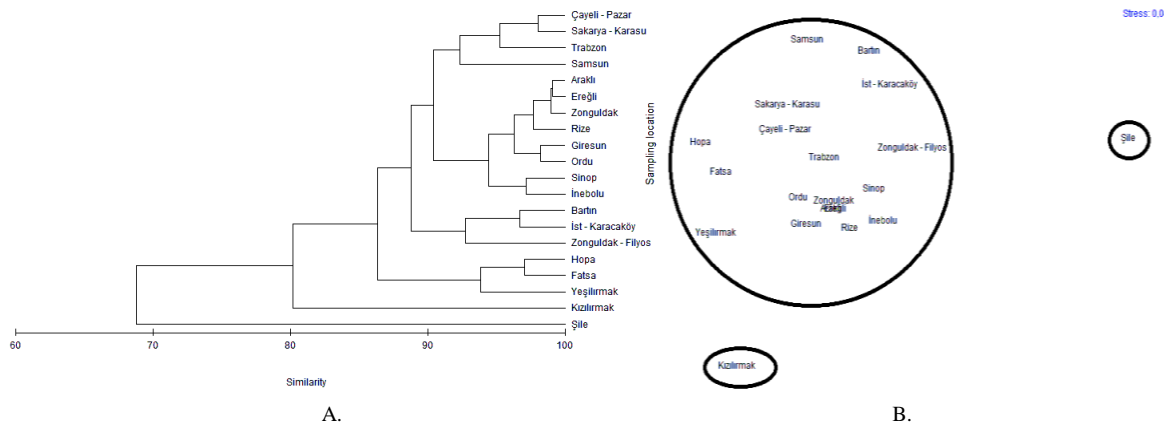
Figure 5. A) Regional Hierarchical Similarity Cluster Analyses and B) MDS analyses results for Synechococcus spp.
