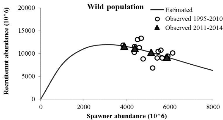
Figure 4. The spawner-recruit relationship of wild Portunus (Portunus) trituberculatus (Miers, 1876) in Zhejiang sea areas. Circle represents the observed data from 1995 to 2010, and triangle represents the observed data from 2011 to 2014.
