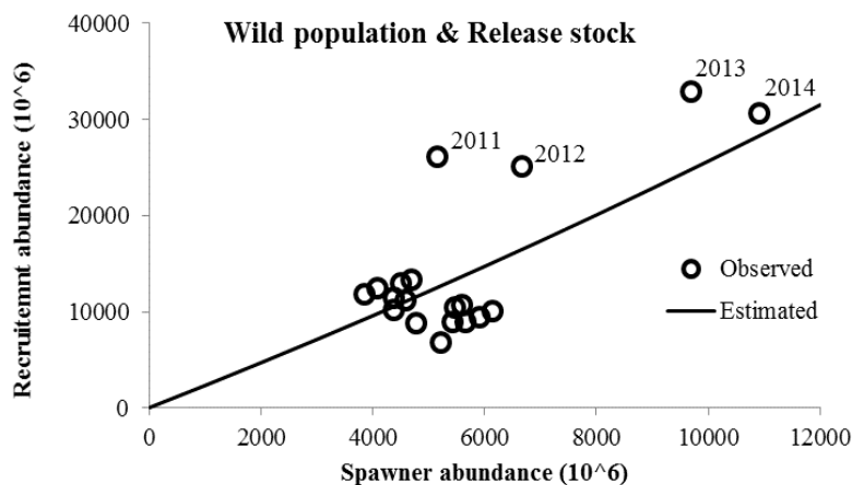
Figure 3. The spawner-recruit relationship of Portunus (Portunus) trituberculatus (Miers, 1876) in Zhejiang sea areas using both wild and release data.
