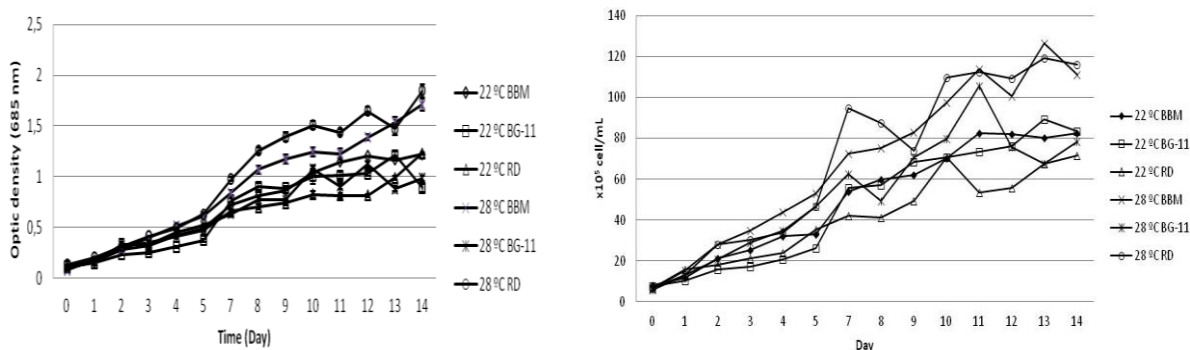
Figure 2. Growth curves of D. protuberans at 22°C and 28°C in BBM, BG-11 and RD medium under a light intensity of 75 µmol m -2 s -1 according to cell number and optic density (685 nm).
